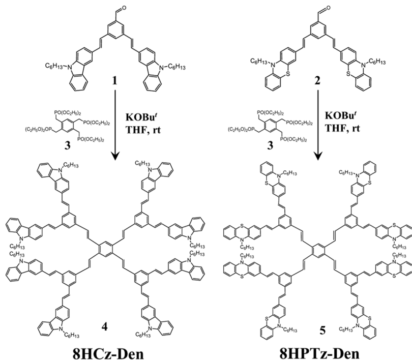
SCHEME 1 Synthetic route for the 8HCz-Den and 8HPTz-Den.
